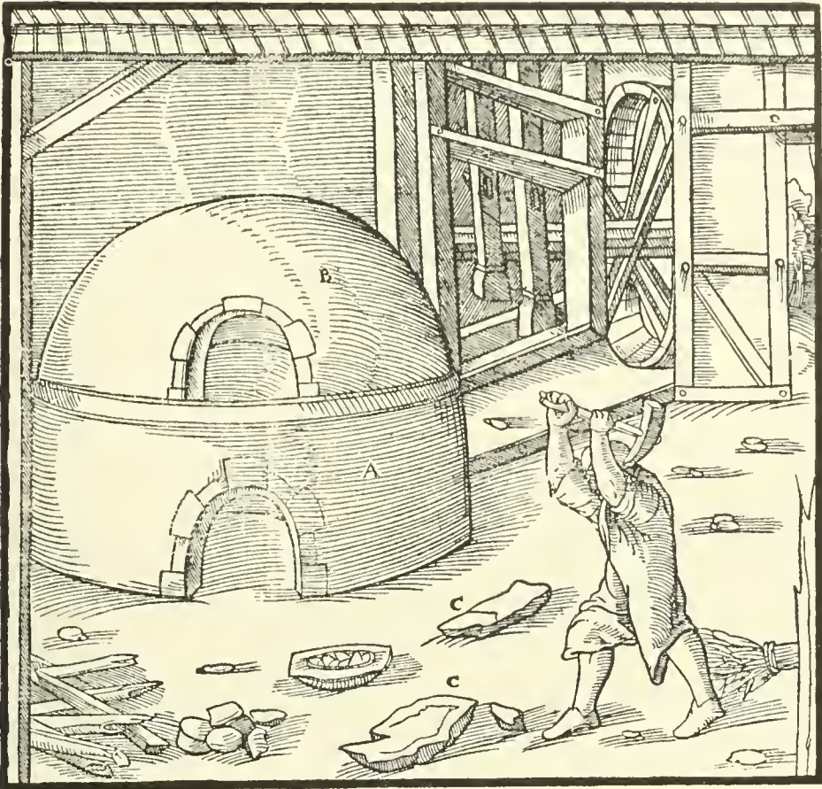
A—LOWER CHAMBER OF THE FIRST FURNACE. B—UPPER CHAMBER. C—VITREOUS MASS.
